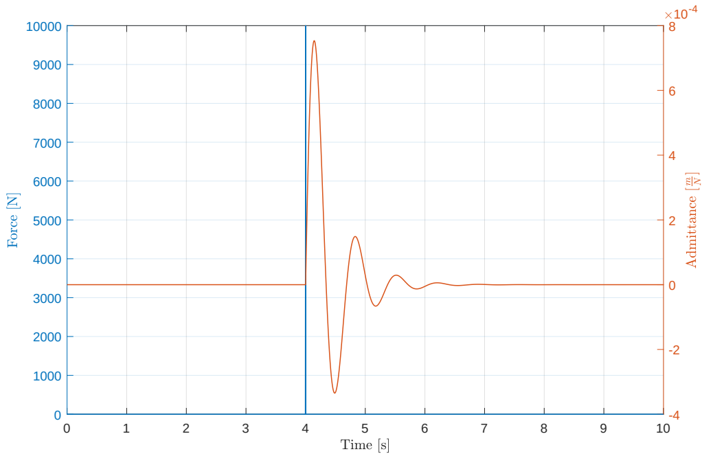
Figure 1: Washing machine impulse response. w_o is 9.4 \frac{\text{radians}}{\text{s}} , w_d is 9.1 \frac{\text{radians}}{\text{s}} , and \zeta is 0.25.
