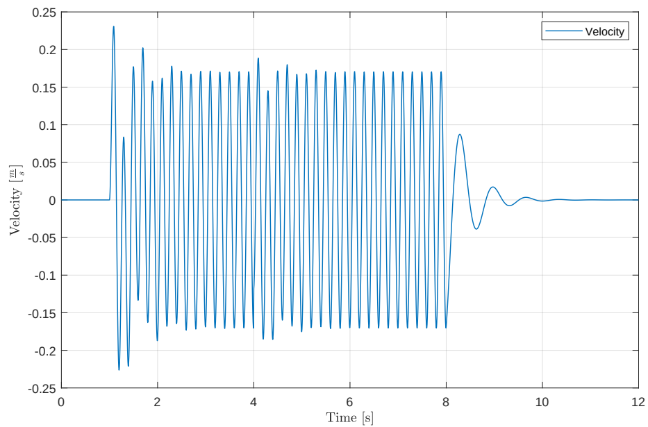
Figure 3: Washing machine velocity response.
