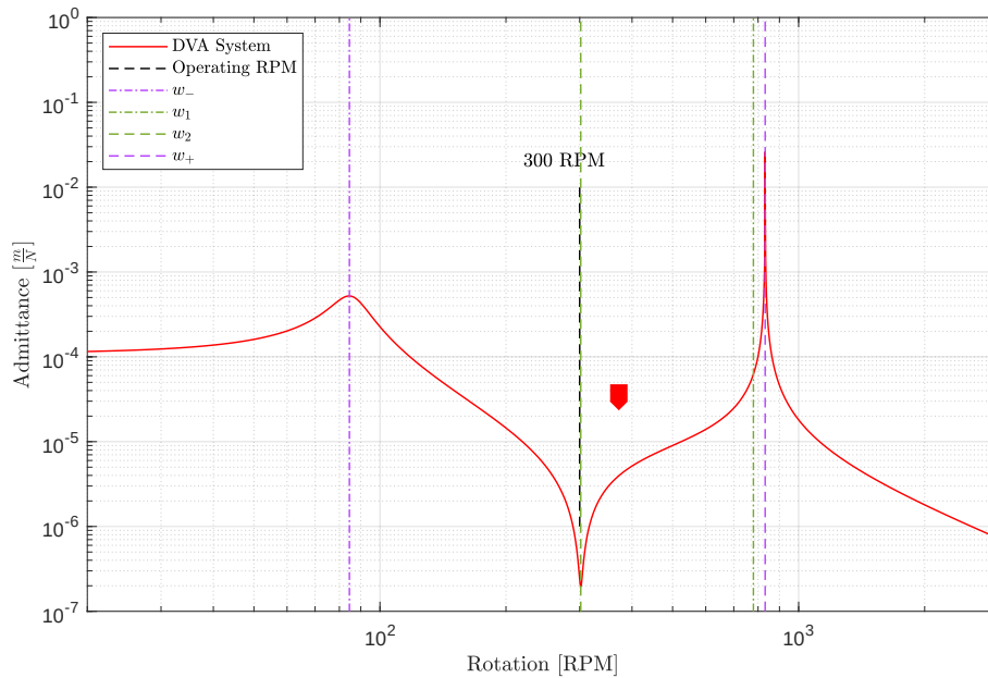
Figure 3: Solution using nDOF script-file function.
