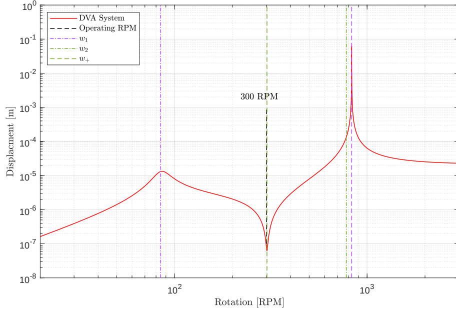
Figure 4: Displacement of the washing machine.
