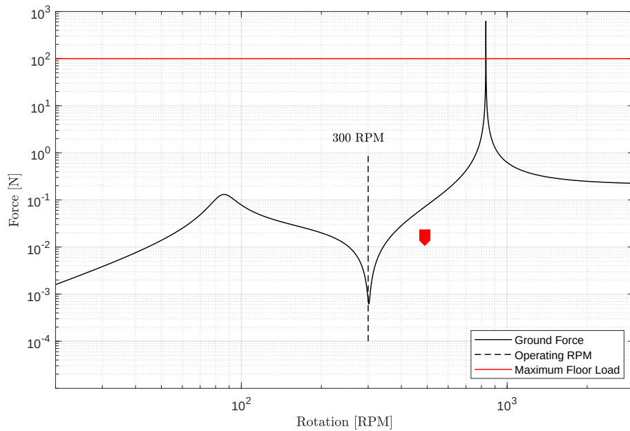
Figure 5: Force applied to the floor.
